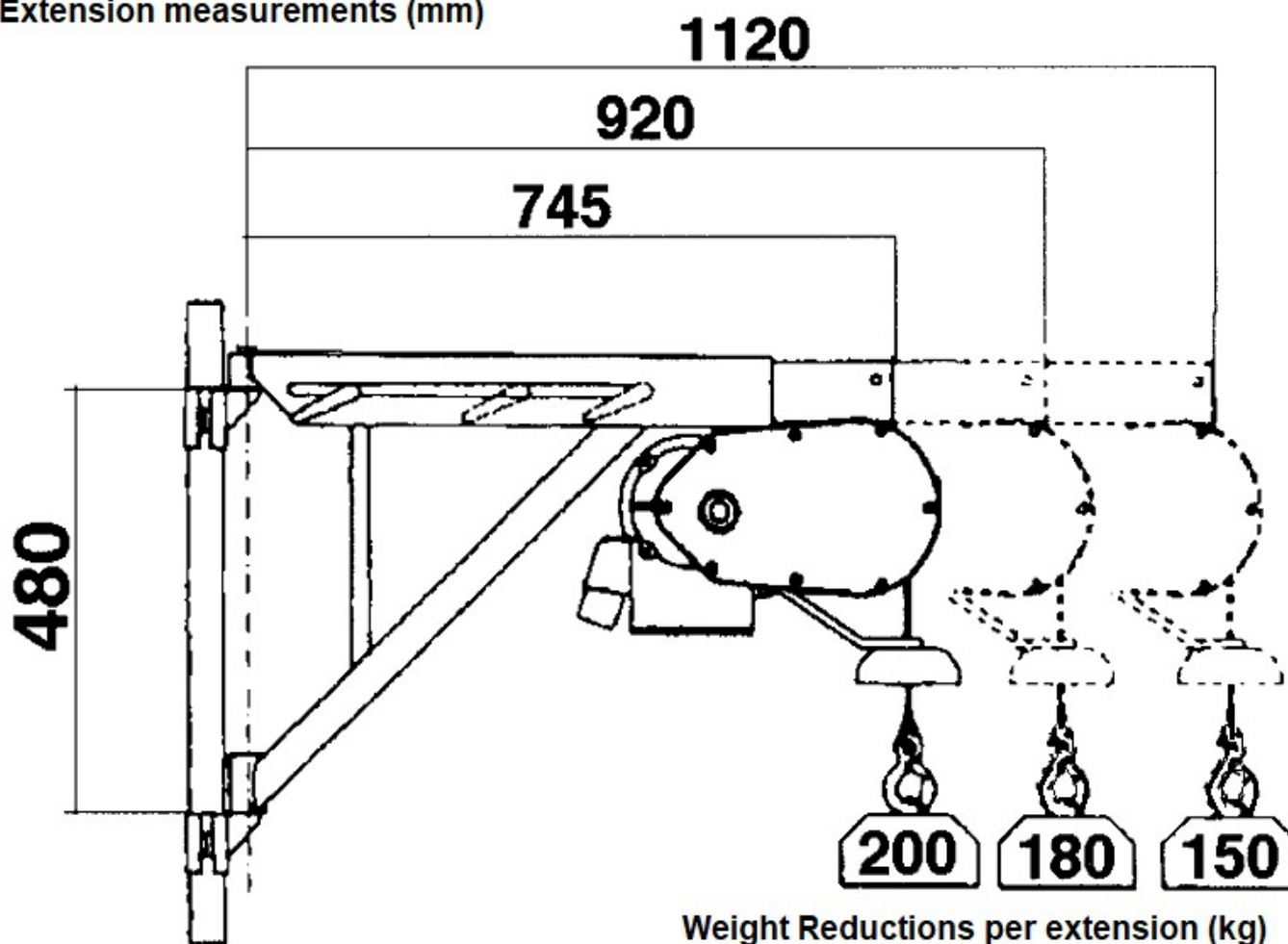
Extension measurements (mm)
